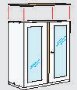
SMALL ALMIRAH (GLASS DOOR) HEIGHT 101cm WIDTH 90cm DEPTH 46cm
